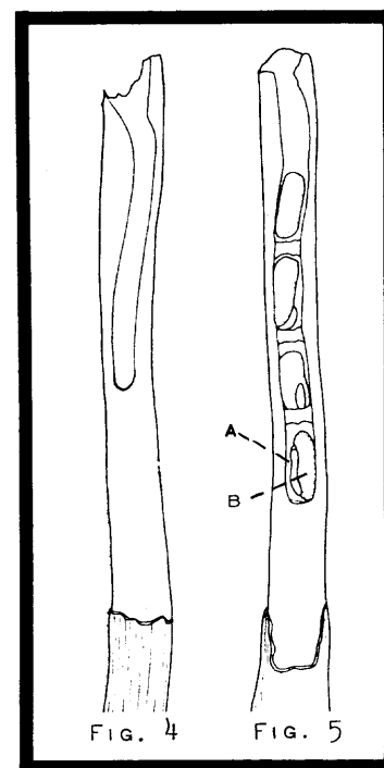
FIG. 4-5. NEST DIAGRAMS OF CERATINA . FIG. 4. OVERWINTERING NEST (HIBERNACULUM). FIG. 5. ACTIVE BROOD NEST (A: BEE LARVA; B: PROVISIONS) (AFTER DALY, 1966)
